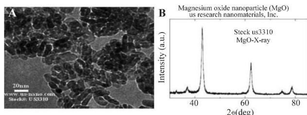
Figure 1. A) Transmission electron microscopy (TEM) image of magnesium oxide nanoparticle. B) X-ray diffraction of magnesium oxide nanoparticles
